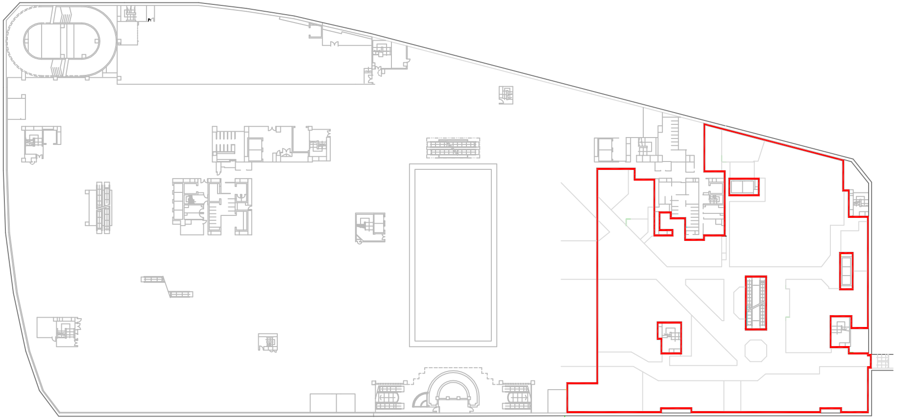
2ND BASEMENT PLAN NGEE ANN CITY
