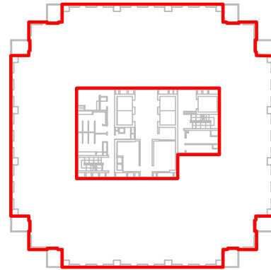
22ND STOREY PLAN TOWER B NGEE ANN CITY
