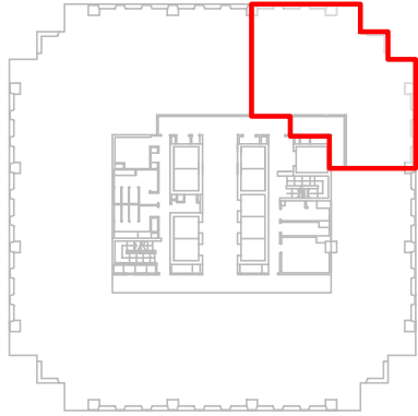
13TH STOREY PLAN TOWER B NGEE ANN CITY
