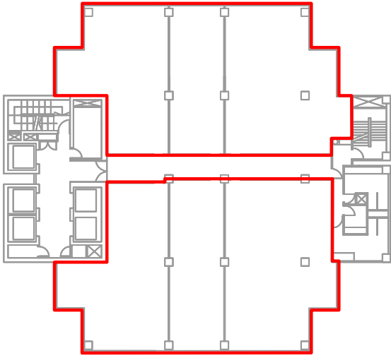
10TH TO 16TH STOREY PLAN WISMA ATRIA
