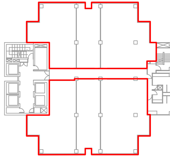
19TH TO 22ND STOREY PLAN WISMA ATRIA
