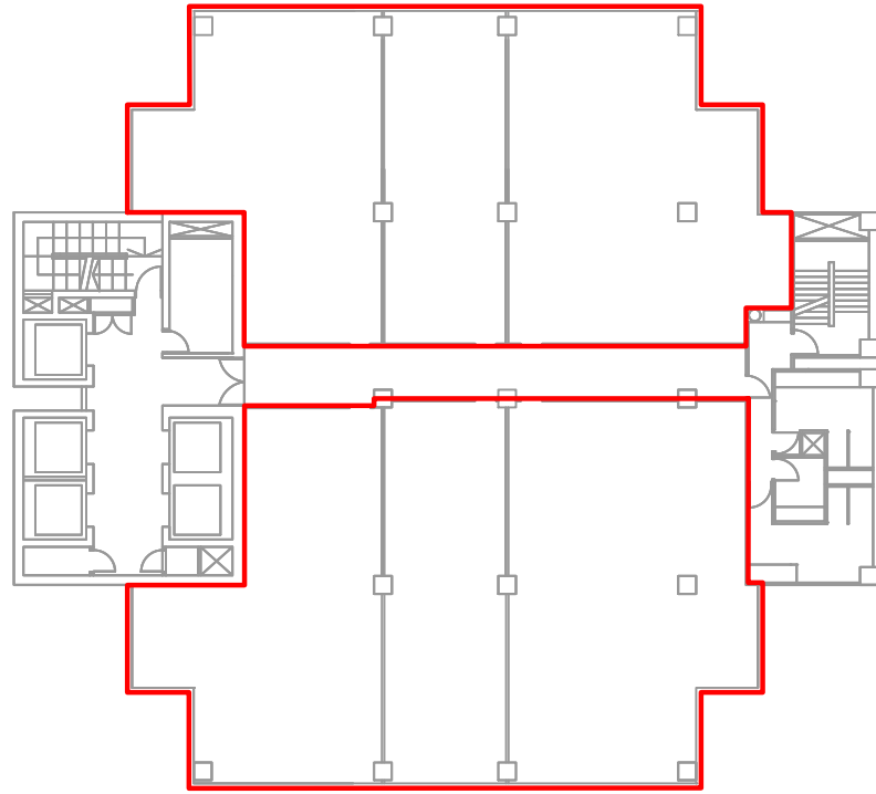
10TH, 11TH, 13TH TO 16TH STOREY PLAN WISMA ATRIA
