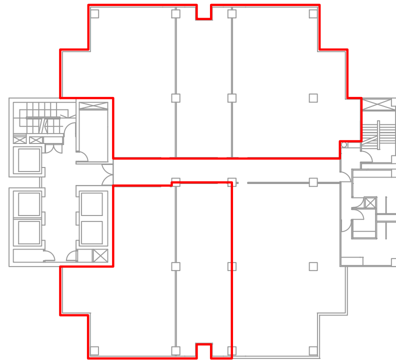
21ST STOREY PLAN WISMA ATRIA
